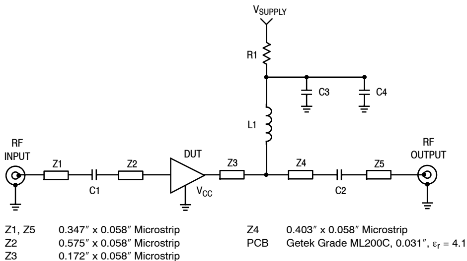
Figure 14. 50 Ohm Test Circuit Schematic
